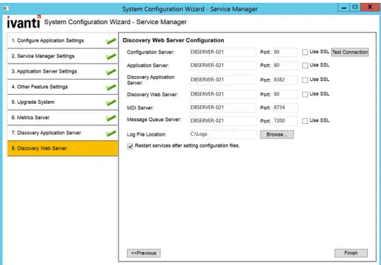
Discovery Web Server Page
