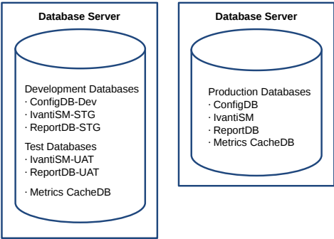
Example of Separate Database Servers
