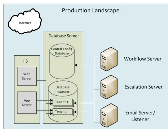
Typical Production Landscape
