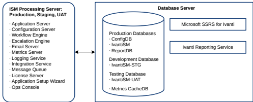
Example of a Single Microsoft SSRS Instance on One Database Server
