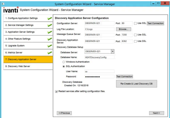
Discovery Application Server Page: No Database
